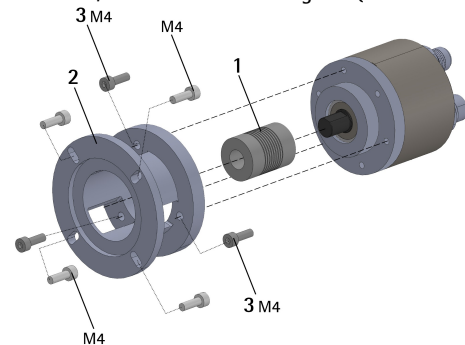
EXM58S, EXO58S with mounting bell (code PF4256)
